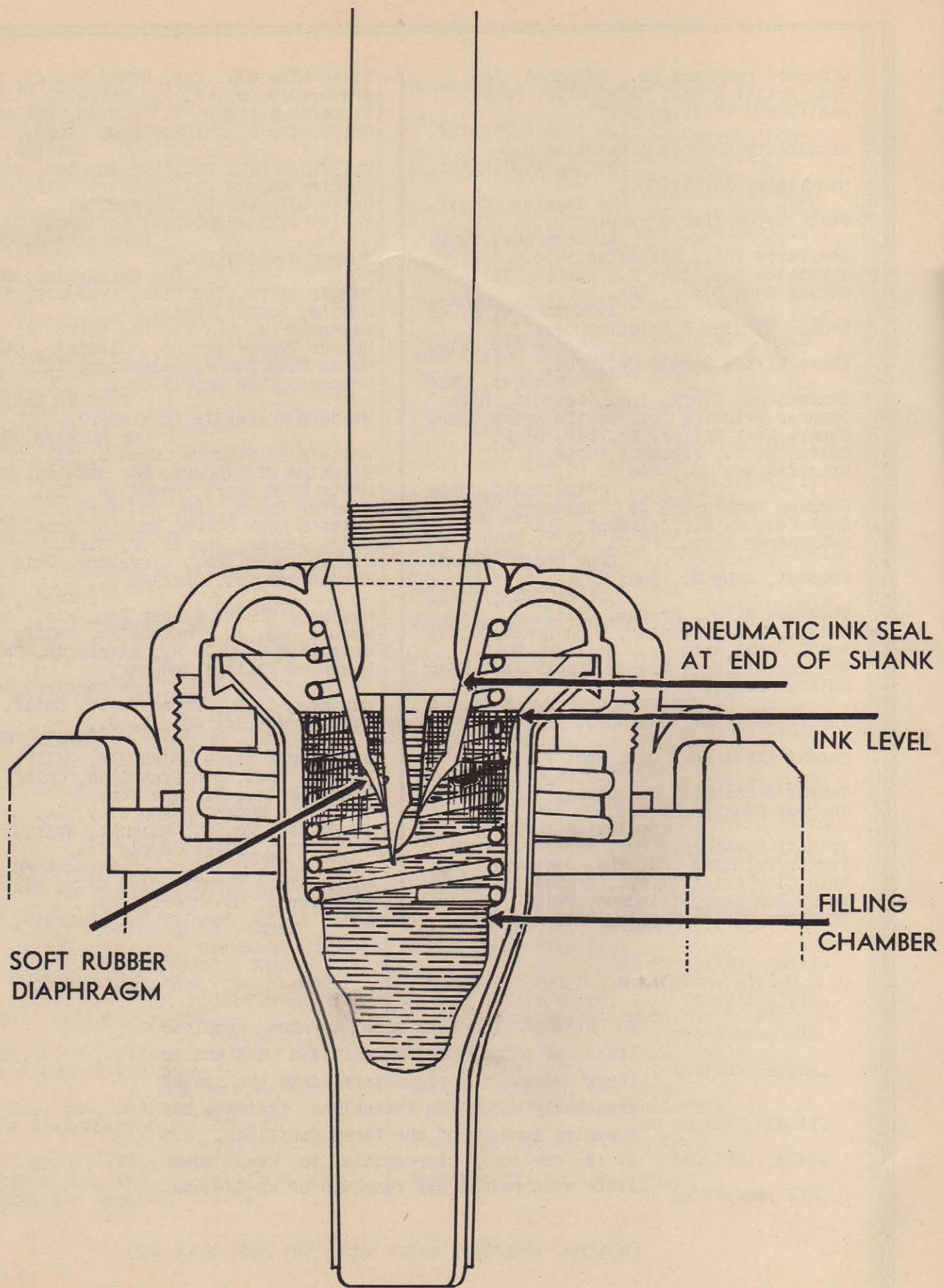
FIRST — Pen Seated in Penfiller.
